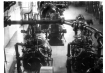
AFC 341-S4-SS1-I21 Horton Street Station - equipment 4. -- 1912. -- 6.5x8.5 glass plate negative. -- Box Number AFC 341-4 AFC 341-18
