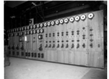
AFC 341-S4-SS1-I19 Horton Street Station - equipment 2. -- 1912. -- 6.5x8.5 glass plate negative. -- Box Number AFC 341-4 AFC 341-18
